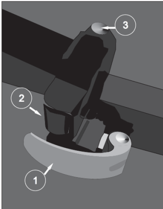
Fig. 1: Closed position 1: Lever 2: Adjustment nut 3: Hinge pin
