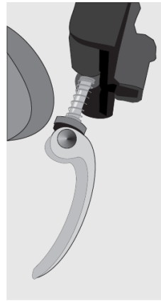
Fig. 1: Closed position 1: Lever 2: Adjustment nut 3: Hinge pin
