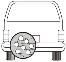
7-pin
